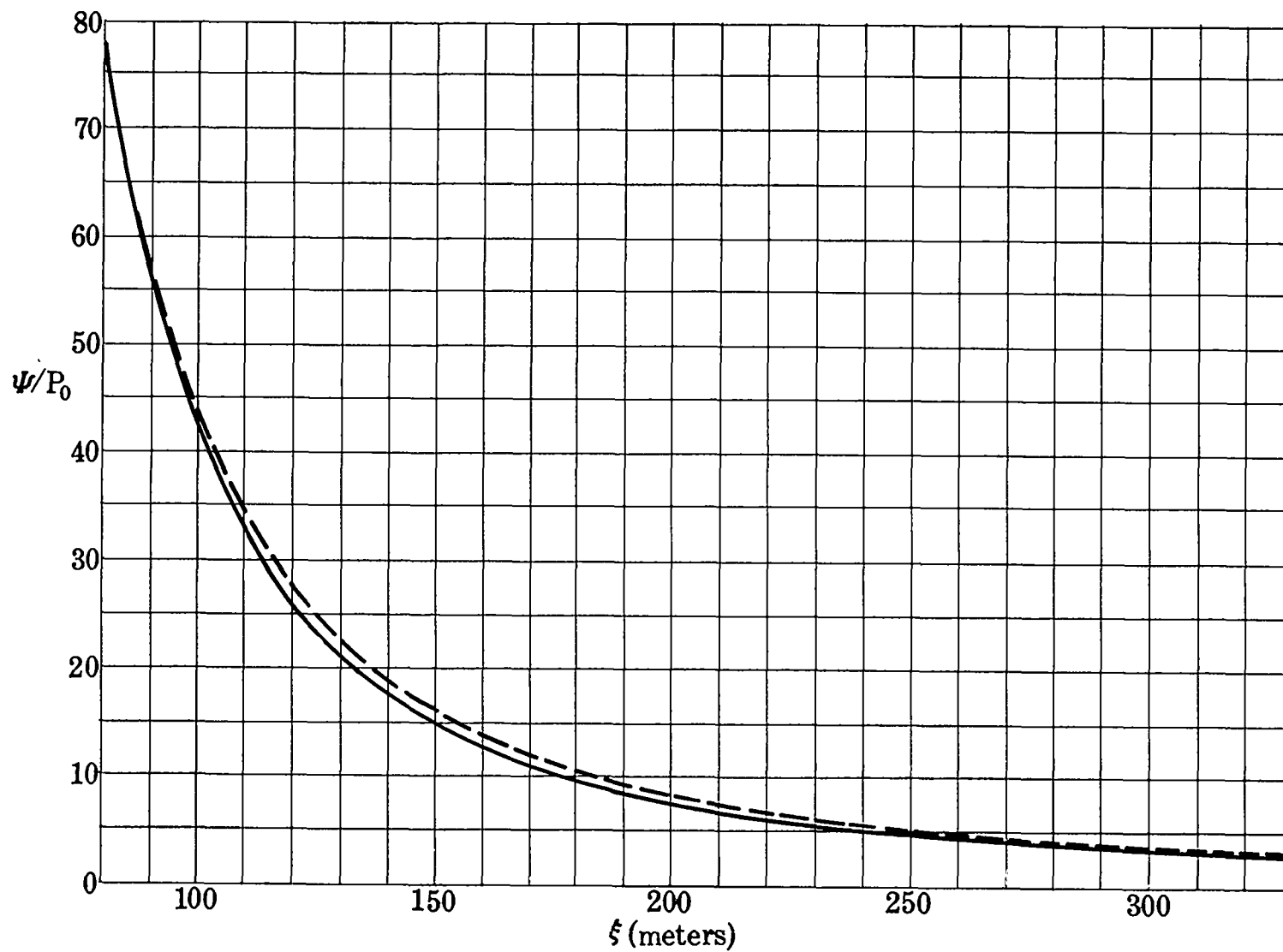
Fig. 9. Shock pressure as a function of shock position; — Problem M, - - - Problem Herman
