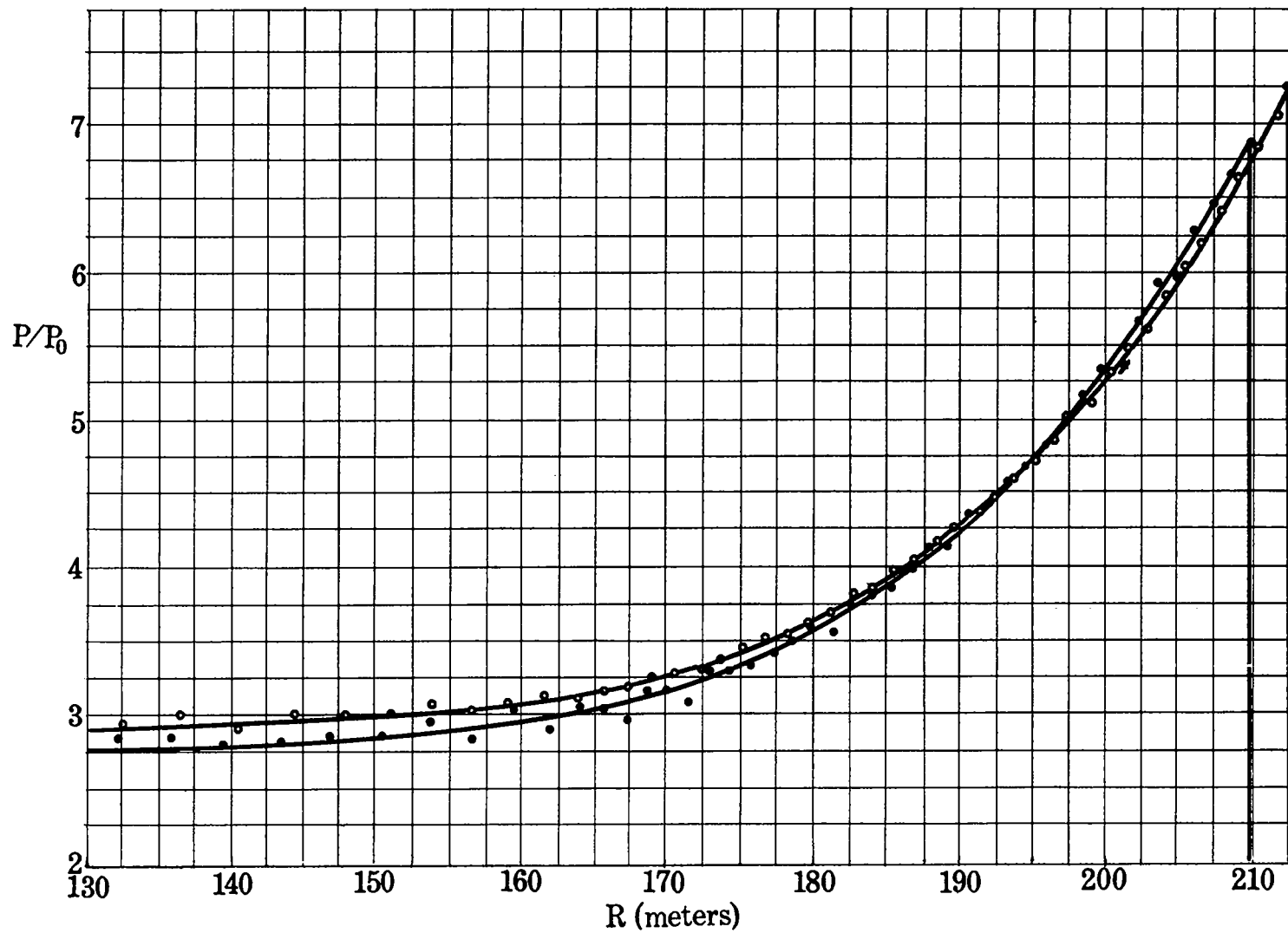
Fig. 6. Pressure as a function of the Eulerian radius at t = 100 milliseconds; • Problem M, ○ Problem Herman
