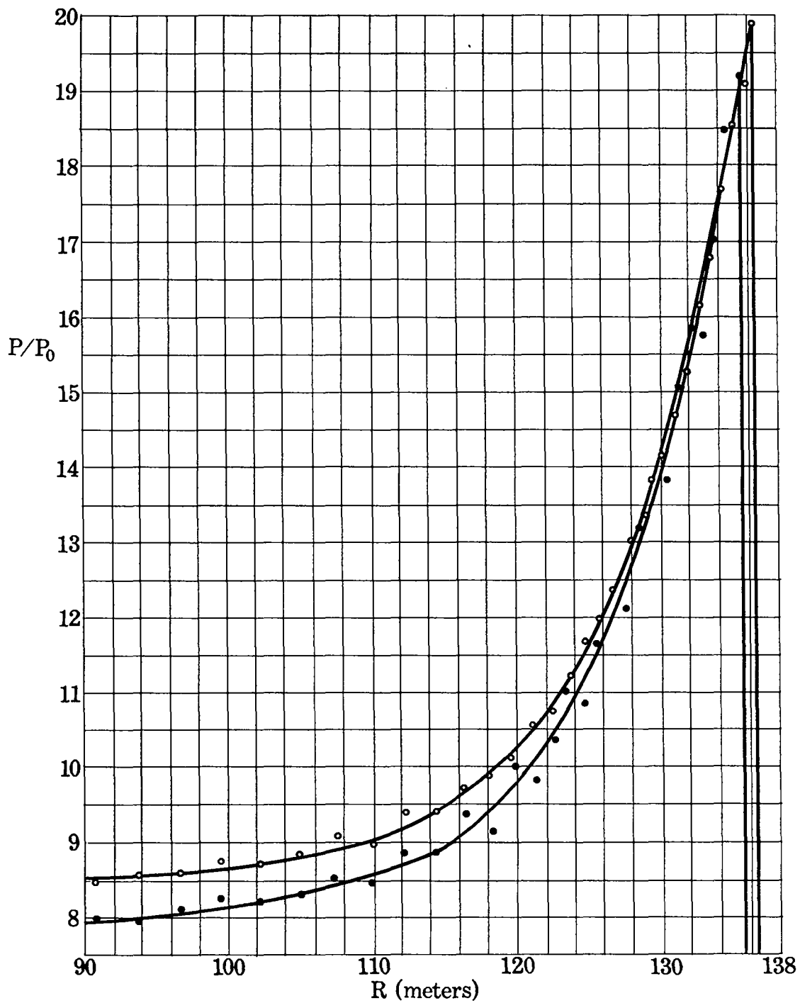
Fig. 4. Pressure as a function of the Eulerian radius at t = 30 milliseconds; \bullet Problem M, \circ Problem Herman
