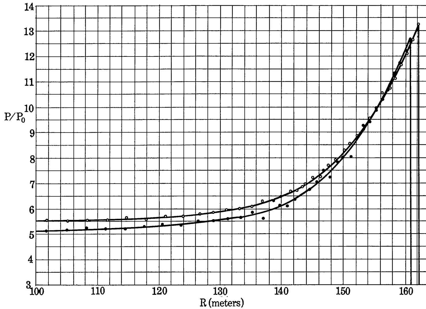
Fig. 5. Pressure as a function of the Eulerian radius at t = 50 milliseconds; \bullet Problem M, \circ Problem Herman
